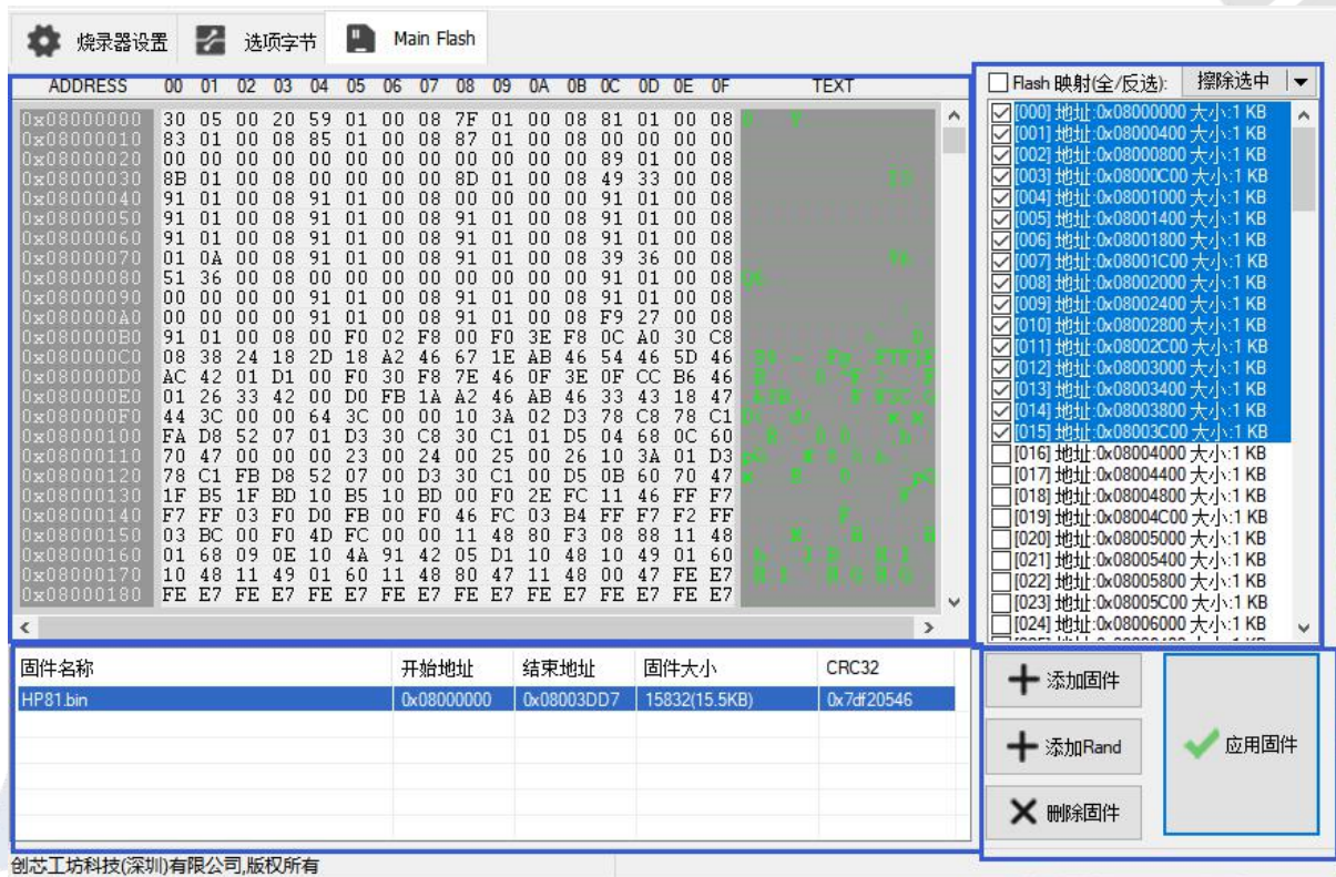
图 3.1.4.3-1 Power Writer Program Memory 标签页
